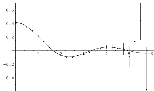
FIGURE 29. The second Fourier coefficient \mu_2 as a function of |A_1| .
