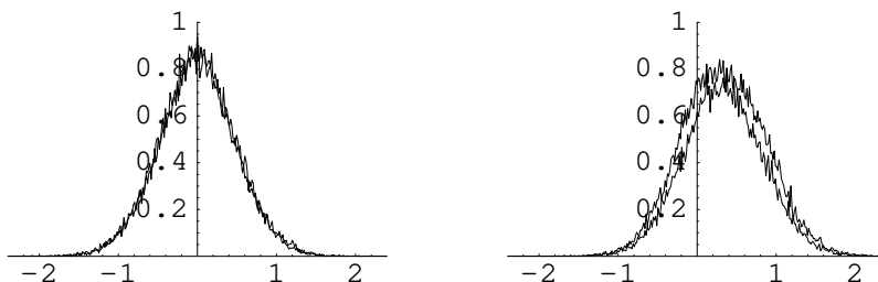
FIGURE 24. The distributions on the left boundary as a function of \mathfrak{R}A_1 (on the left) and of \mathfrak{S}A_1 (on the right).
