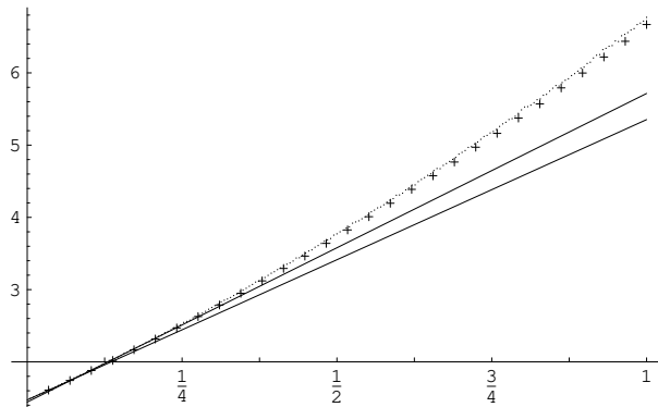
FIGURE 3. The numbers \hat{\omega}_k for 59 \times 401 and 397 \times 793 with the horizontal axis scaled proportionately to 1/LV .
