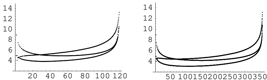
FIGURE 49. The correlation \left\langle (h(p) - h(0)) \right\rangle_{\mu_{FK}}^2 - \frac{2}{3} \ln|p| on disks of radii 60 and 180.
