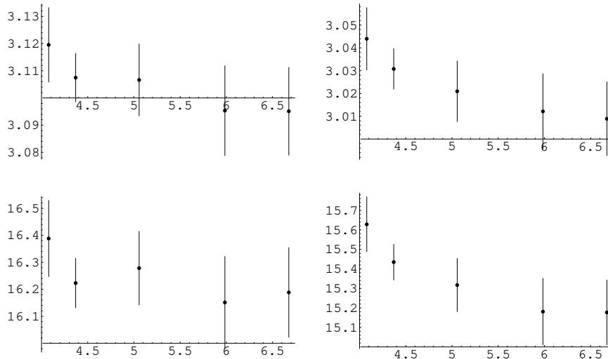
FIGURE 6. The quotients \widehat{\mu}_{1,i}^L/\widehat{\sigma}_1^i and \widehat{\mu}_{8,i}^L/\widehat{\sigma}_8^i for i = 4 and 6 as functions of \log LV .
