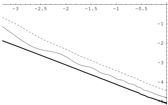
FIGURE 11. Log-Log plot of \langle \sigma(\theta_1)\sigma(\theta_2) \rangle and of \langle e^{i(\phi(\theta_1) - \phi(\theta_2))} \rangle as functions of \sin((\theta_1 - \theta_2)/2) for the cylinder 397 \times 793 . (See text.)
