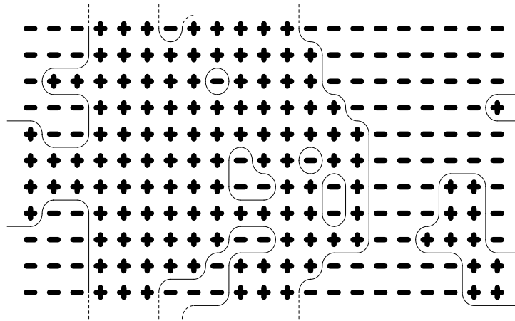
FIGURE 57. A configuration on an 11 \times 21 cylinder with the jump lines of h .
