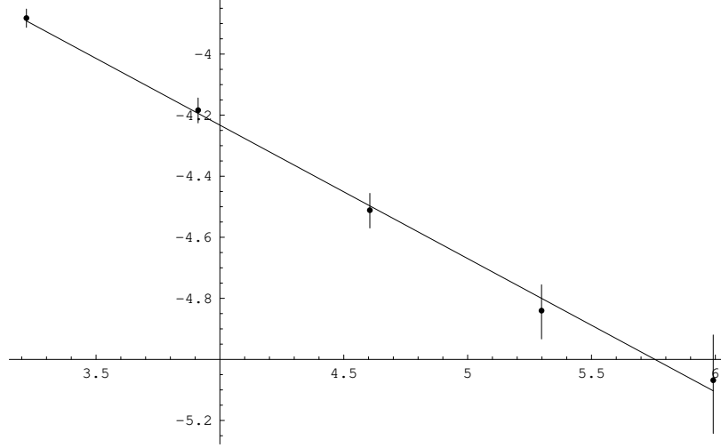
FIGURE 30. Log-log plot of 1 - \pi_h - \pi_v measured on a square as a function of the linear number of sites.
