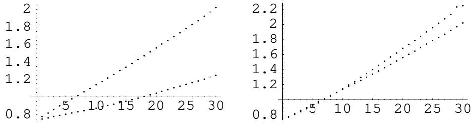
FIGURE 54. The numbers \hat{\omega}_k at infinite temperature.
