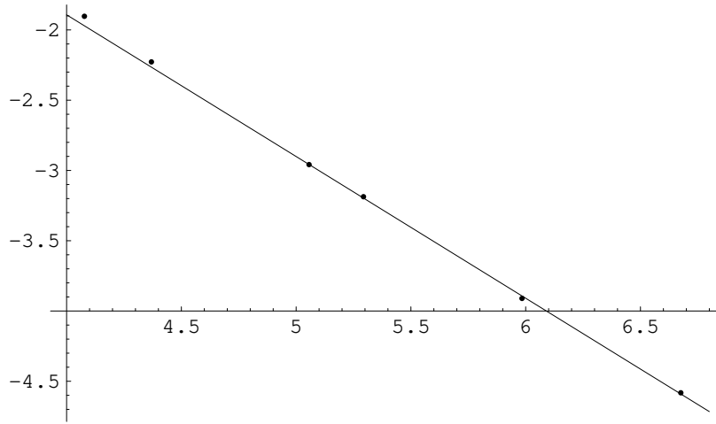
FIGURE 4. Log-Log plot of the slopes of the linear fit of \hat{\omega}_k as a function of LV .
