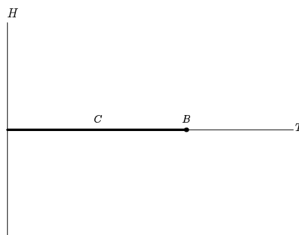
FIGURE 2.2b. Qualitative phase diagram for a ferromagnet.
