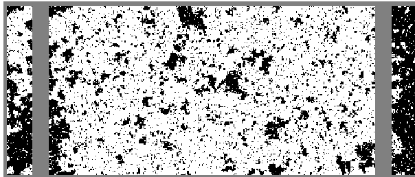
FIGURE 18. Configurations on cylinders.
