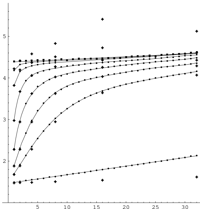
FIGURE 16. The \widehat{\omega}_k , k \in \{1, 2, \dots, 32\} on a disk ( + ) and on a cylinder ( \bullet and \blacksquare ) for various inner circles.
