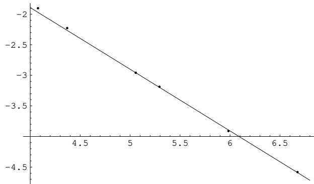
FIGURE 4. Log-Log plot of the slopes of the linear fit of \widehat{\omega}_k as a function of LV .
