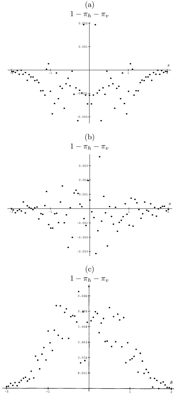
FIGURE 4. The difference (1 - \pi_h - \pi_v) as a function of s : (a) percolation by sites on a square lattice, (b) percolation by sites on a triangular lattice, (c) percolation by bonds on a triangular lattice.
