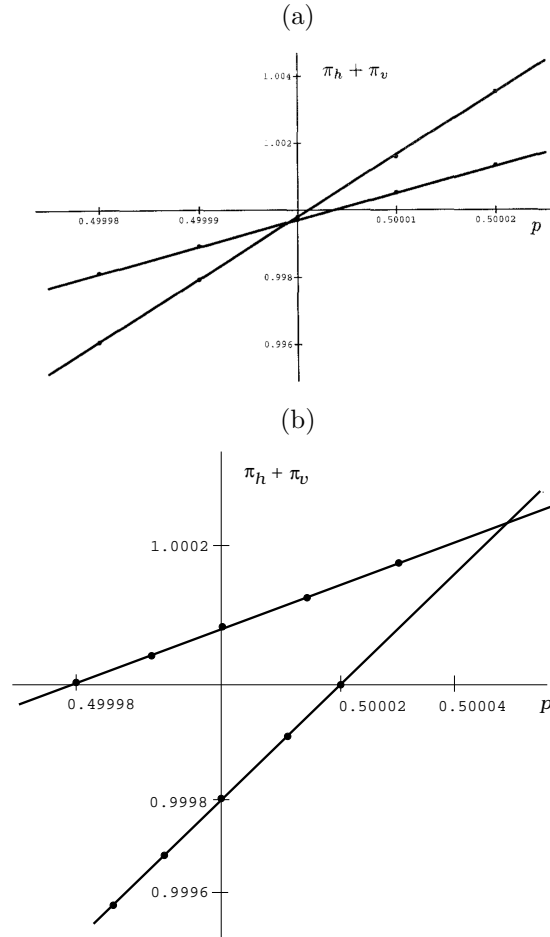
FIGURE 2. Numerical determination of p_c for the percolation by sites on a triangular lattice: (a) for the lattices with s \sim 0 , (b) for the lattices with s \sim \ln 5 .
