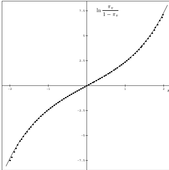
FIGURE 3. The four crossing probability functions for the percolation by bonds on a hexagonal lattice (dots) and by sites on a square lattice (curve): (a) \ln \frac{\pi_h}{1 - \pi_h} , (b) \ln \frac{\pi_v}{1 - \pi_v} , (c) \ln \pi_{hv} , (d) \ln \pi_d .
