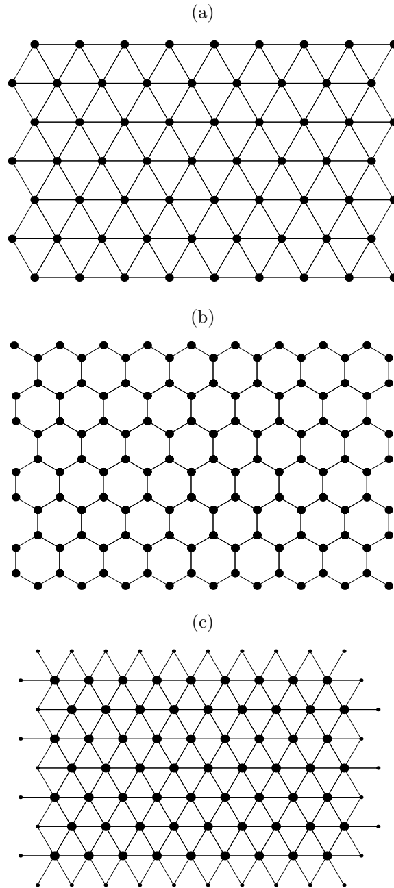
FIGURE 1. (a) A triangular lattice with (\text{width}, \text{height})=(5,4) , (b) a hexagonal lattice with (\text{width}, \text{height}) = (10, 5) , (c) a triangular lattice with (\text{width}, \text{height}) = (4, 3) for the percolation by bonds.
