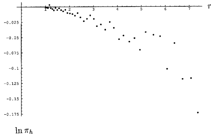
FIGURE 5. Asymptotic behavior of \ln \pi_h .
